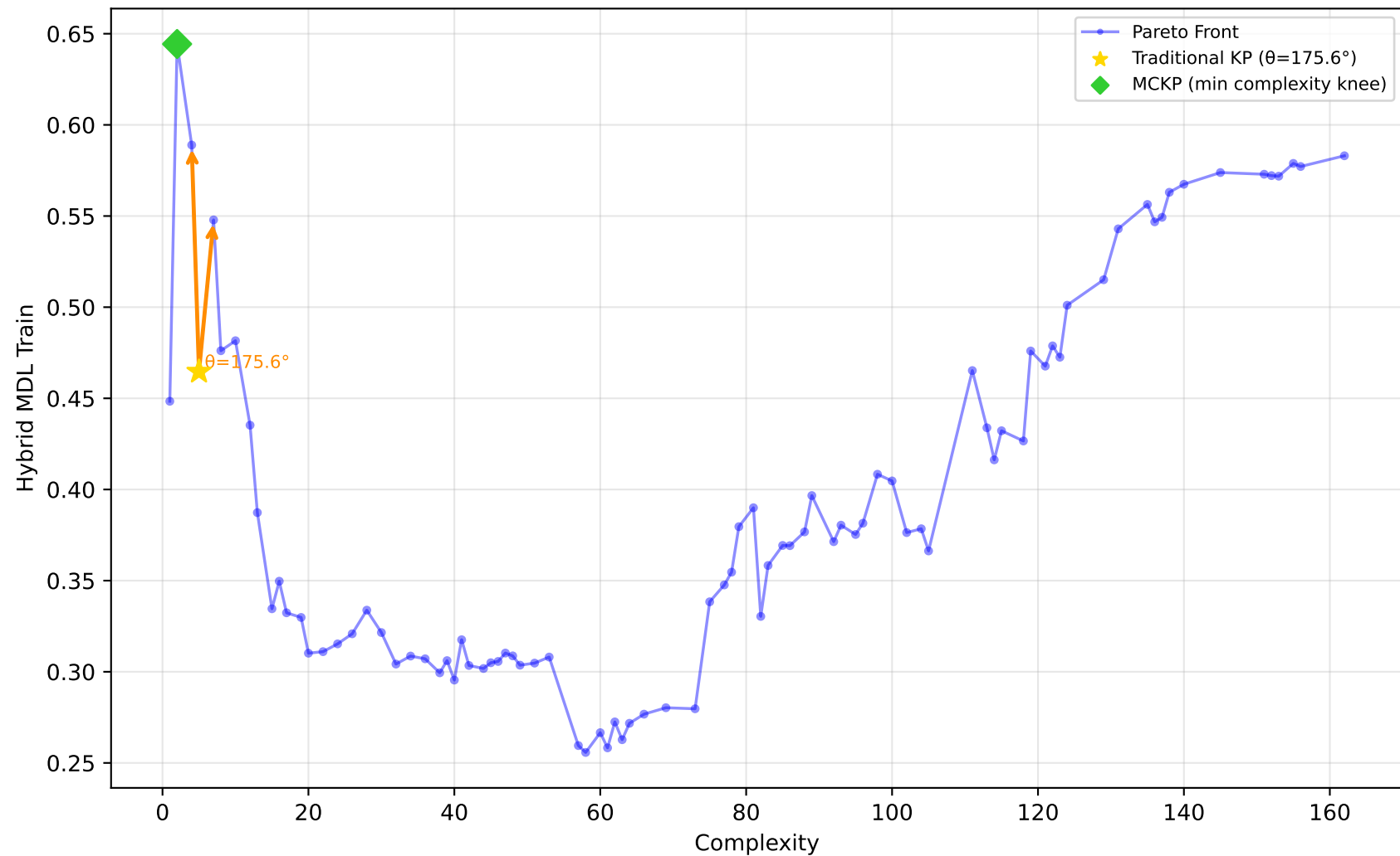
561_cpu - Run 20 - MVP - Hybrid MDL Train \lambda_1=0.50, \lambda_2=0.20, \lambda_3=0.00 | Difficulty: 1.00 | Method: hmr
