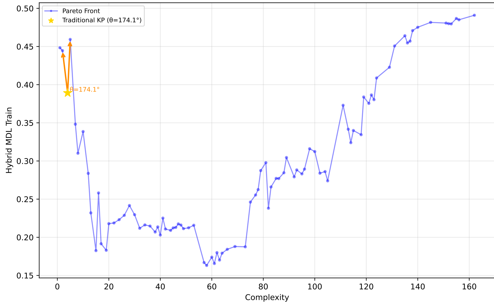
561_cpu - Run 20 - MVP - Hybrid MDL Train \lambda_1=0.70, \lambda_2=0.00, \lambda_3=0.10 | Difficulty: 1.00 | Method: hmr
