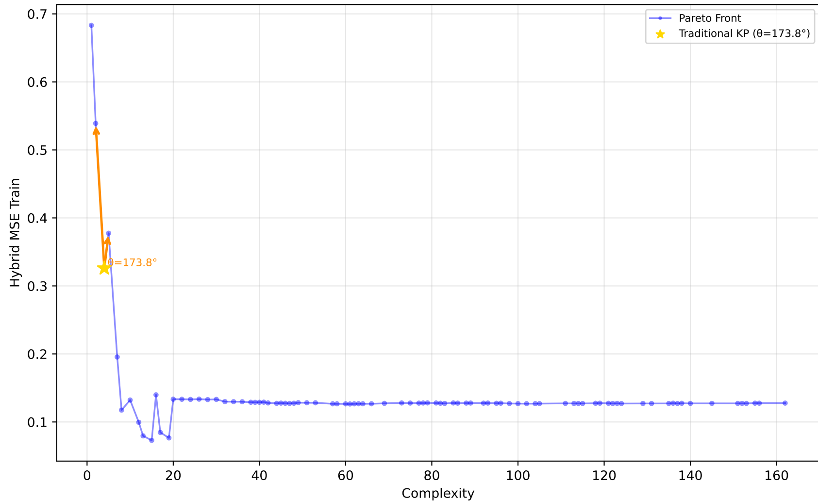
561_cpu - Run 20 - MVP - Hybrid MSE Train \lambda_1=0.70, \lambda_2=0.00, \lambda_3=0.10 | Difficulty: 1.00 | Method: hmr
