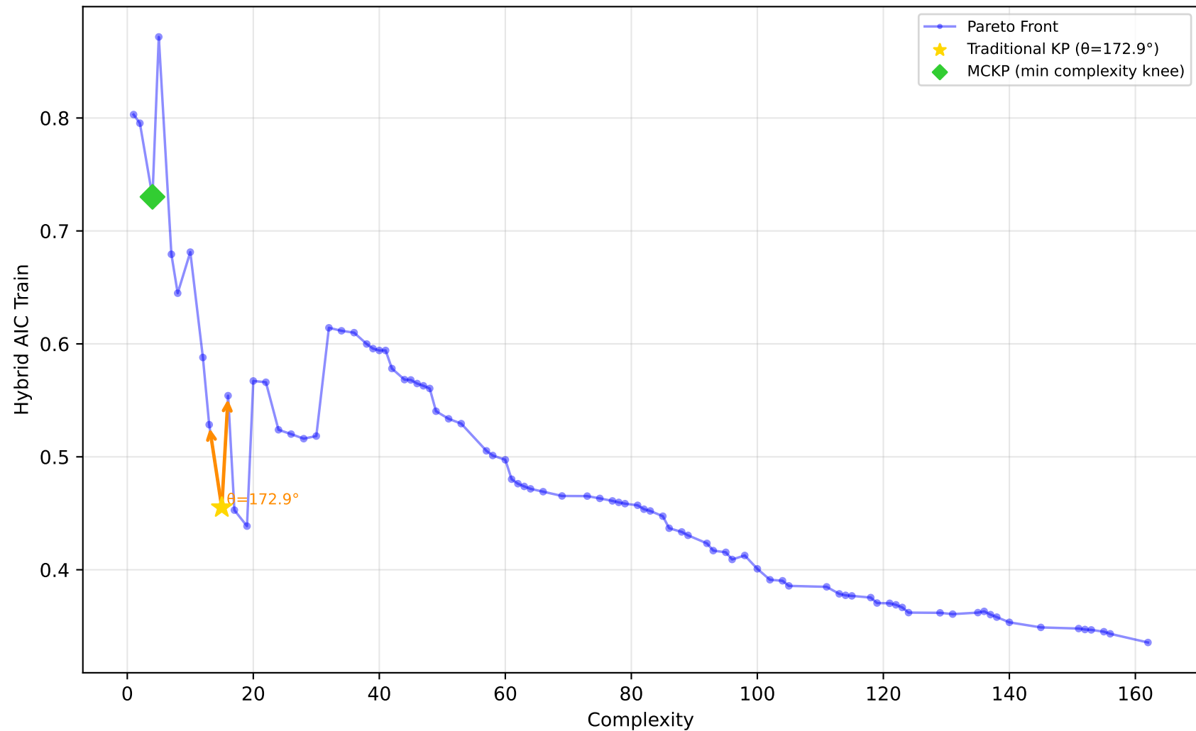
561_cpu - Run 20 - SVP - Hybrid AIC Train \lambda_1=0.90, \lambda_2=0.00, \lambda_3=0.30 | Difficulty: 1.00 | Method: hmr
