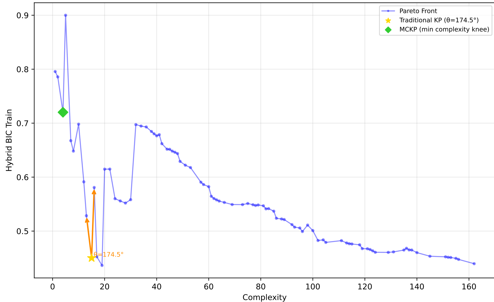
561_cpu - Run 20 - SVP - Hybrid BIC Train \lambda_1=1.00, \lambda_2=0.00, \lambda_3=0.40 | Difficulty: 1.00 | Method: hmr
