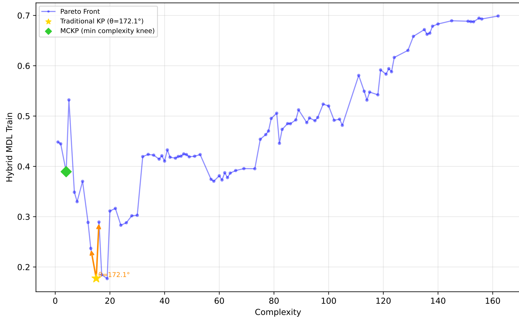
561_cpu - Run 20 - SVP - Hybrid MDL Train \lambda_1=0.90, \lambda_2=0.00, \lambda_3=0.30 | Difficulty: 1.00 | Method: hmr
