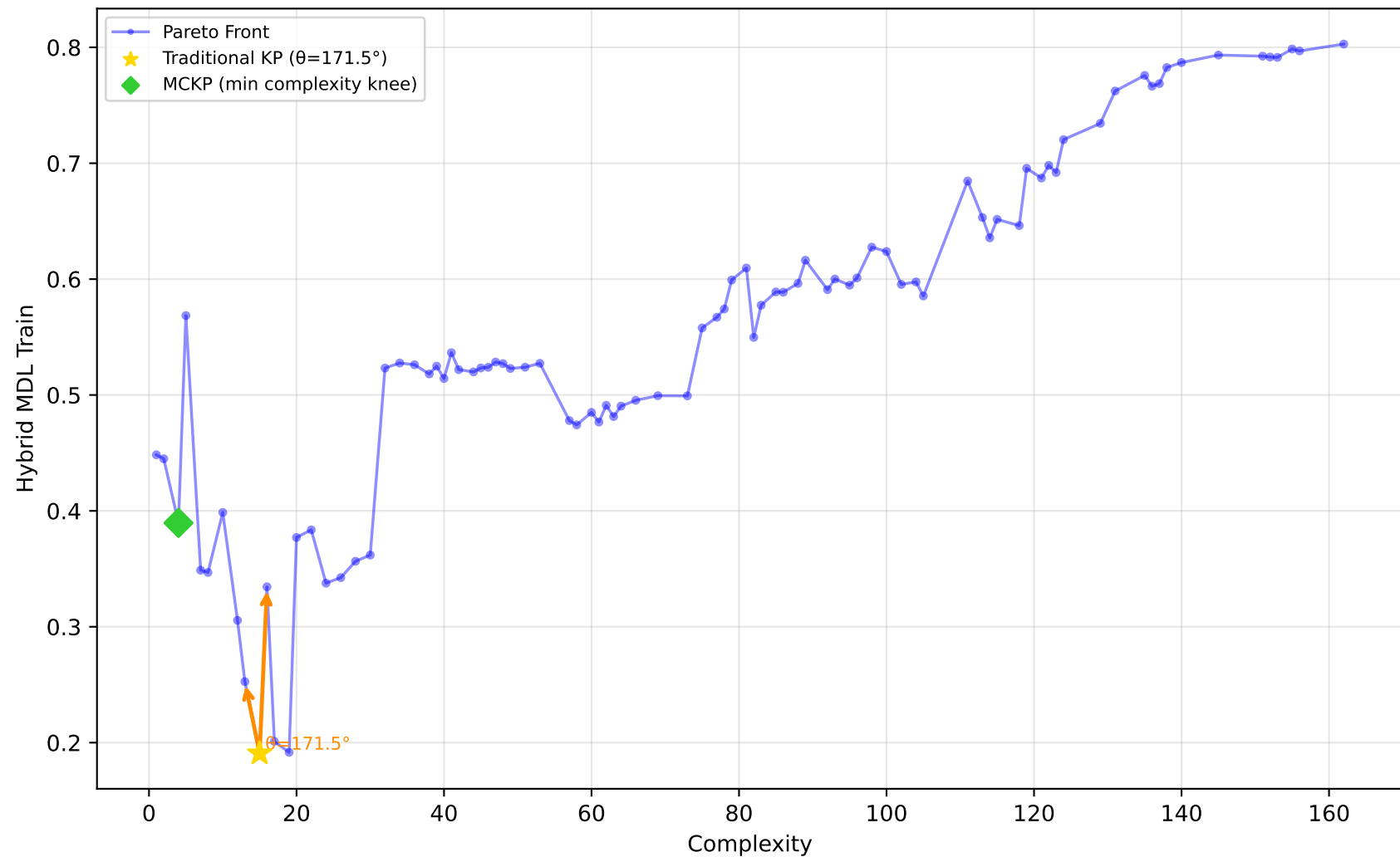
561_cpu - Run 20 - SVP - Hybrid MDL Train \lambda_1=1.00, \lambda_2=0.00, \lambda_3=0.40 | Difficulty: 1.00 | Method: hmr
