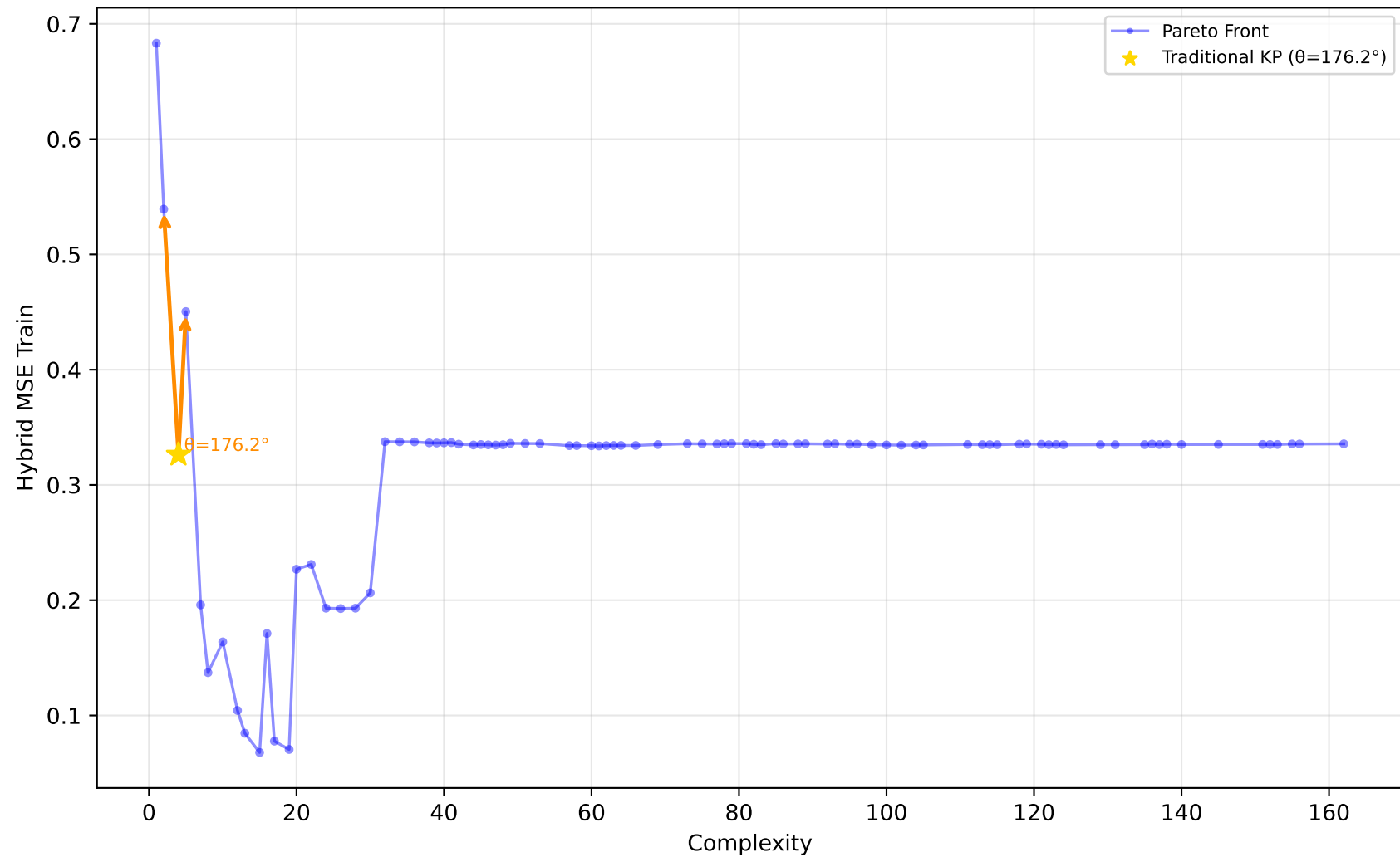
561_cpu - Run 20 - SVP - Hybrid MSE Train \lambda_1=0.90, \lambda_2=0.00, \lambda_3=0.30 | Difficulty: 1.00 | Method: hmr
