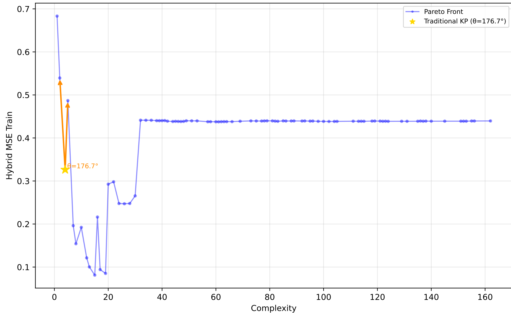
561_cpu - Run 20 - SVP - Hybrid MSE Train \lambda_1=1.00, \lambda_2=0.00, \lambda_3=0.40 | Difficulty: 1.00 | Method: hmr
