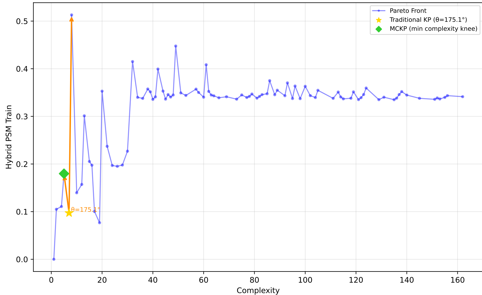
561_cpu - Run 20 - SVP - Hybrid PSM Train \lambda_1=0.90, \lambda_2=0.00, \lambda_3=0.30 | Difficulty: 1.00 | Method: hmr
