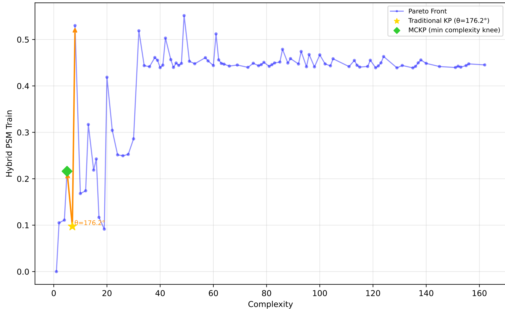
561_cpu - Run 20 - SVP - Hybrid PSM Train \lambda_1=1.00, \lambda_2=0.00, \lambda_3=0.40 | Difficulty: 1.00 | Method: hmr
