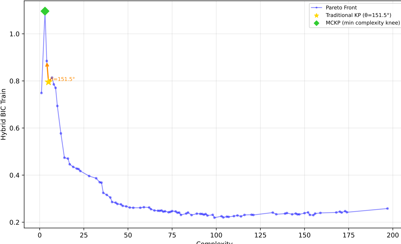
561_cpu - Run 21 - MVP - Hybrid BIC Train \lambda_1=0.70, \lambda_2=0.00, \lambda_3=0.10 | Difficulty: 1.00 | Method: hmr
