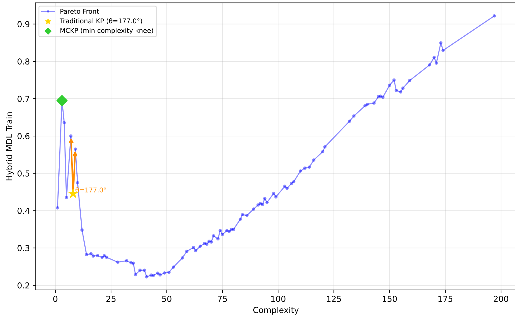
561_cpu - Run 21 - MVP - Hybrid MDL Train \lambda_1=0.50, \lambda_2=0.20, \lambda_3=0.00 | Difficulty: 1.00 | Method: hmr
