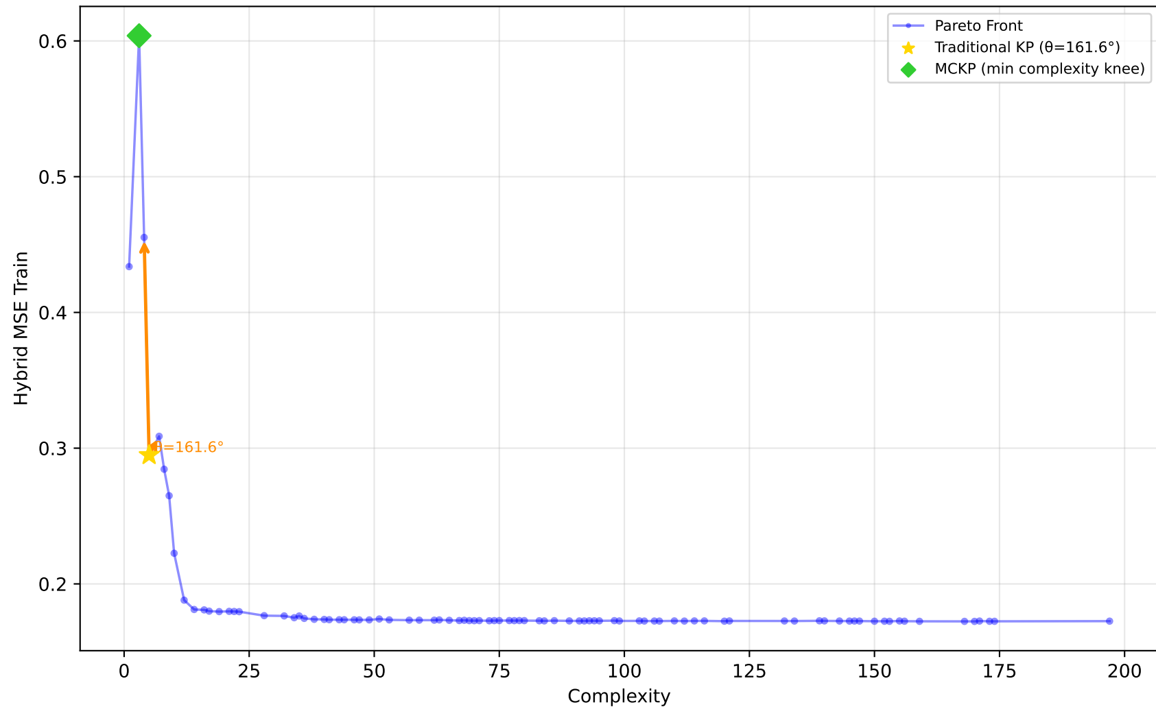
561_cpu - Run 21 - MVP - Hybrid MSE Train \lambda_1=0.70, \lambda_2=0.00, \lambda_3=0.10 | Difficulty: 1.00 | Method: hmr
