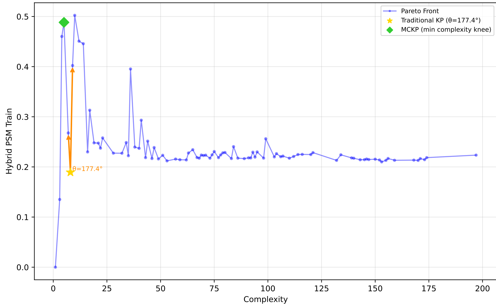
561_cpu - Run 21 - MVP - Hybrid PSM Train \lambda_1=0.50, \lambda_2=0.20, \lambda_3=0.00 | Difficulty: 1.00 | Method: hmr
