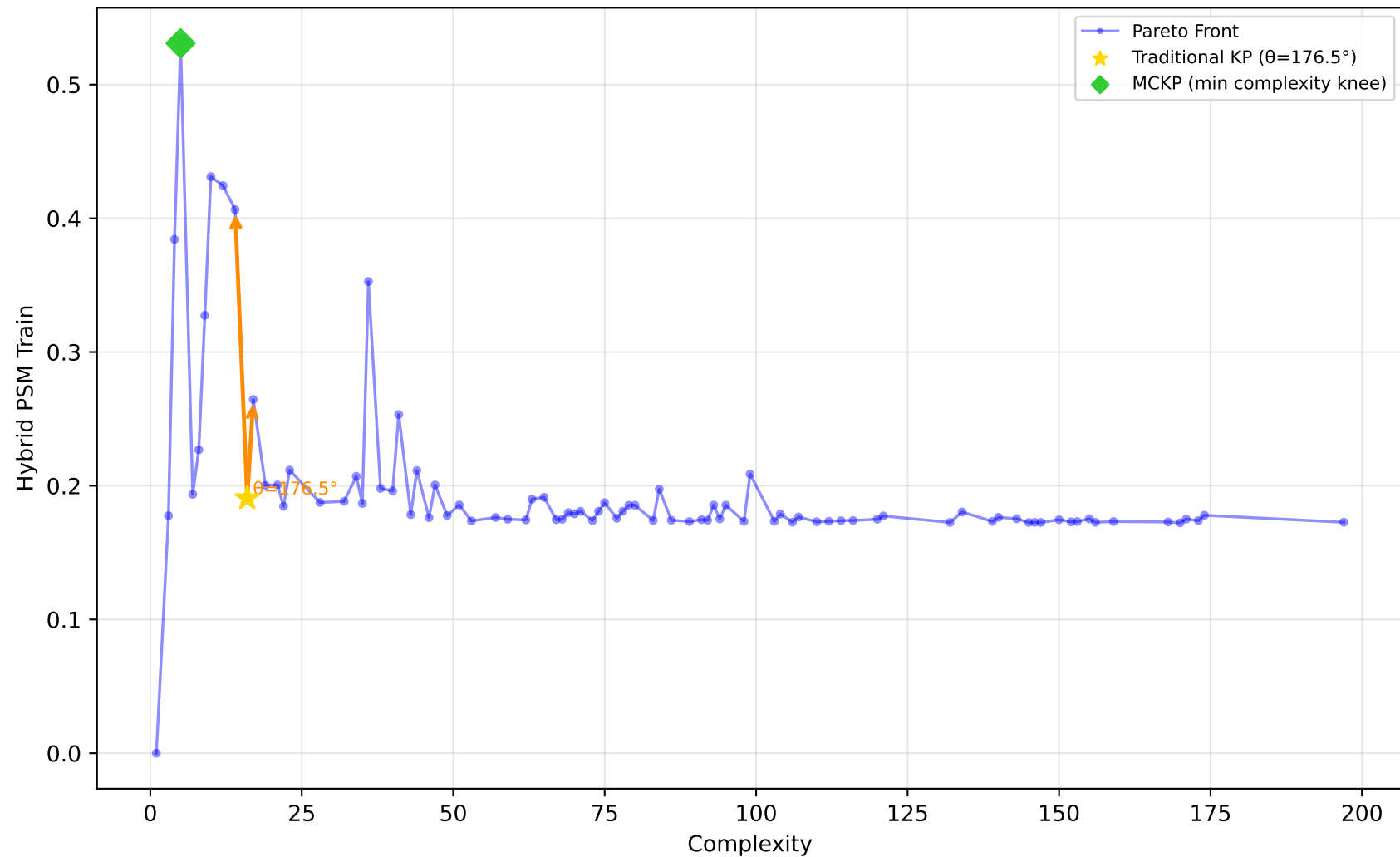
561_cpu - Run 21 - MVP - Hybrid PSM Train \lambda_1=0.70, \lambda_2=0.00, \lambda_3=0.10 | Difficulty: 1.00 | Method: hmr
