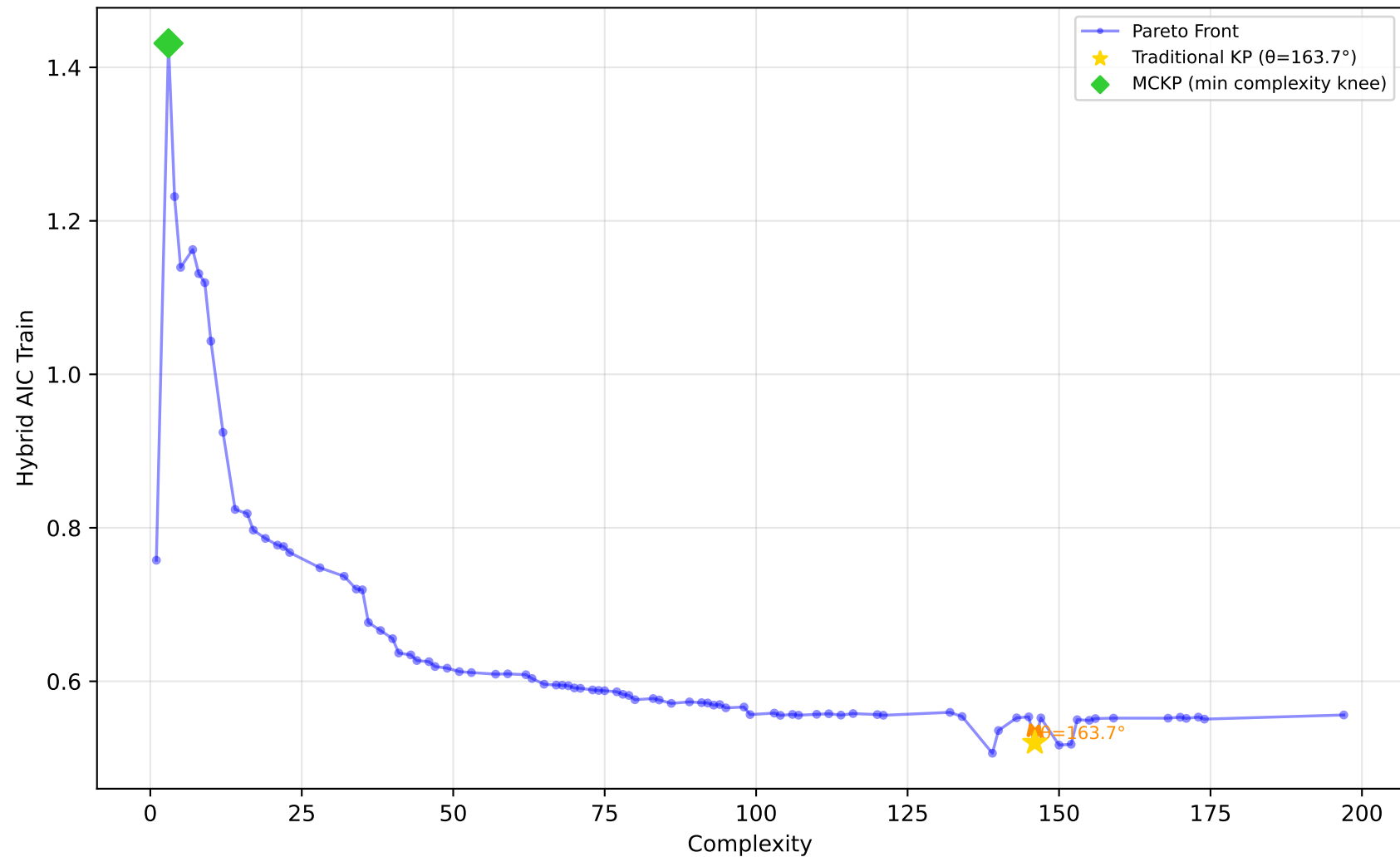
561_cpu - Run 21 - SVP - Hybrid AIC Train \lambda_1=1.00, \lambda_2=0.00, \lambda_3=0.40 | Difficulty: 1.00 | Method: hmr
