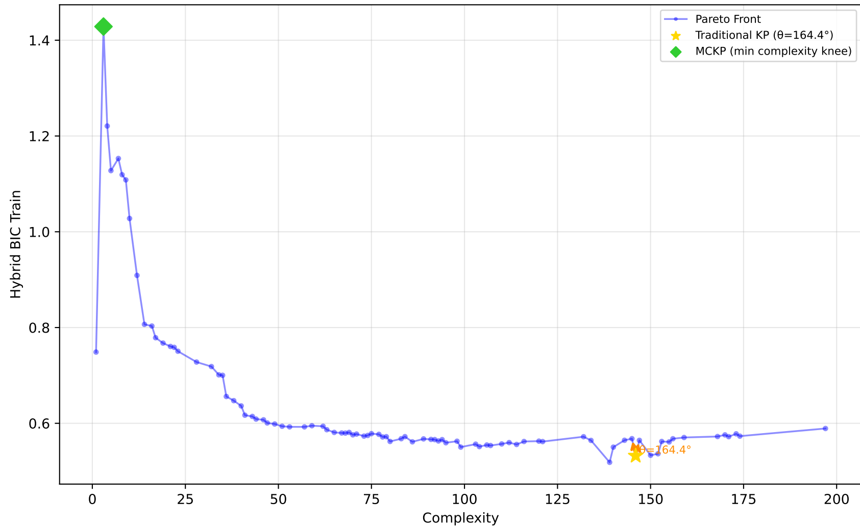
561_cpu - Run 21 - SVP - Hybrid BIC Train \lambda_1=1.00, \lambda_2=0.00, \lambda_3=0.40 | Difficulty: 1.00 | Method: hmr
