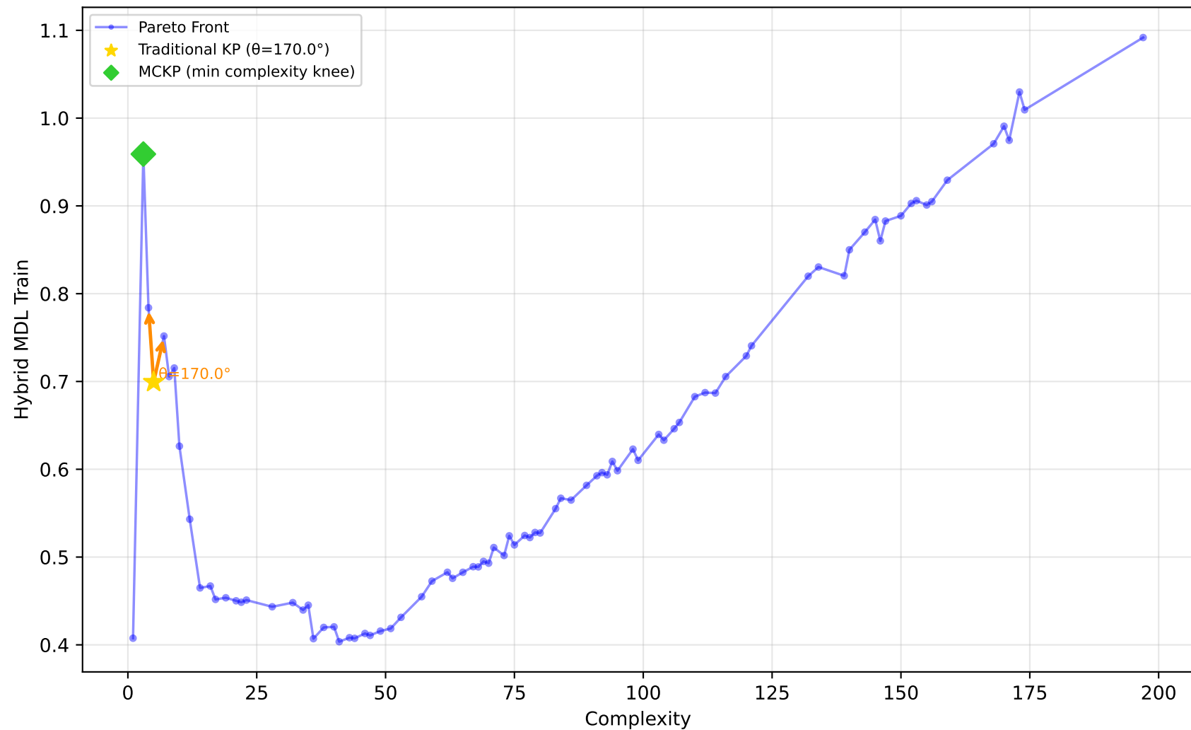
561_cpu - Run 21 - SVP - Hybrid MDL Train \lambda_1=0.90, \lambda_2=0.00, \lambda_3=0.30 | Difficulty: 1.00 | Method: hmr
