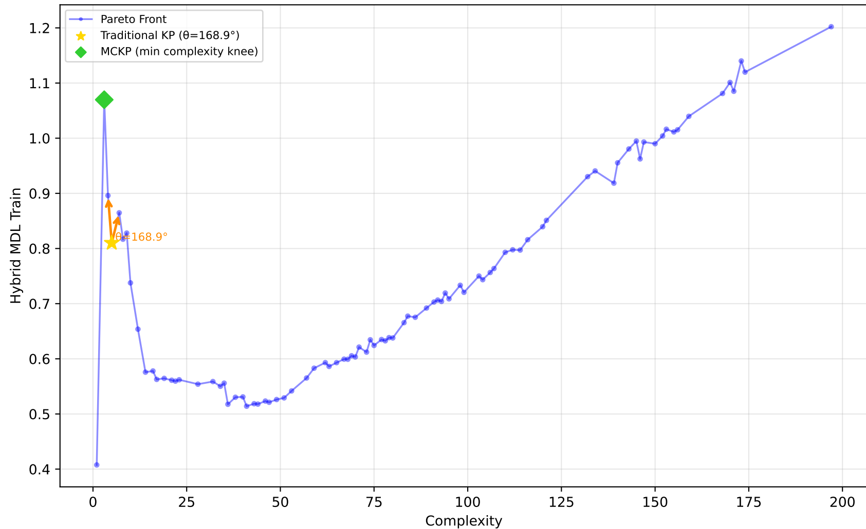
561_cpu - Run 21 - SVP - Hybrid MDL Train \lambda_1=1.00, \lambda_2=0.00, \lambda_3=0.40 | Difficulty: 1.00 | Method: hmr
