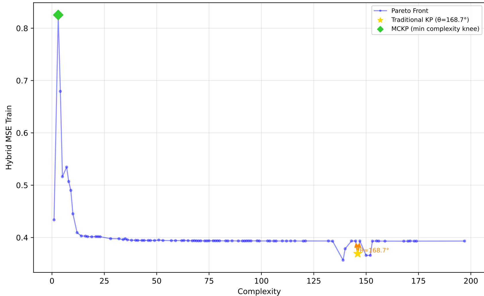
561_cpu - Run 21 - SVP - Hybrid MSE Train \lambda_1=0.90, \lambda_2=0.00, \lambda_3=0.30 | Difficulty: 1.00 | Method: hmr
