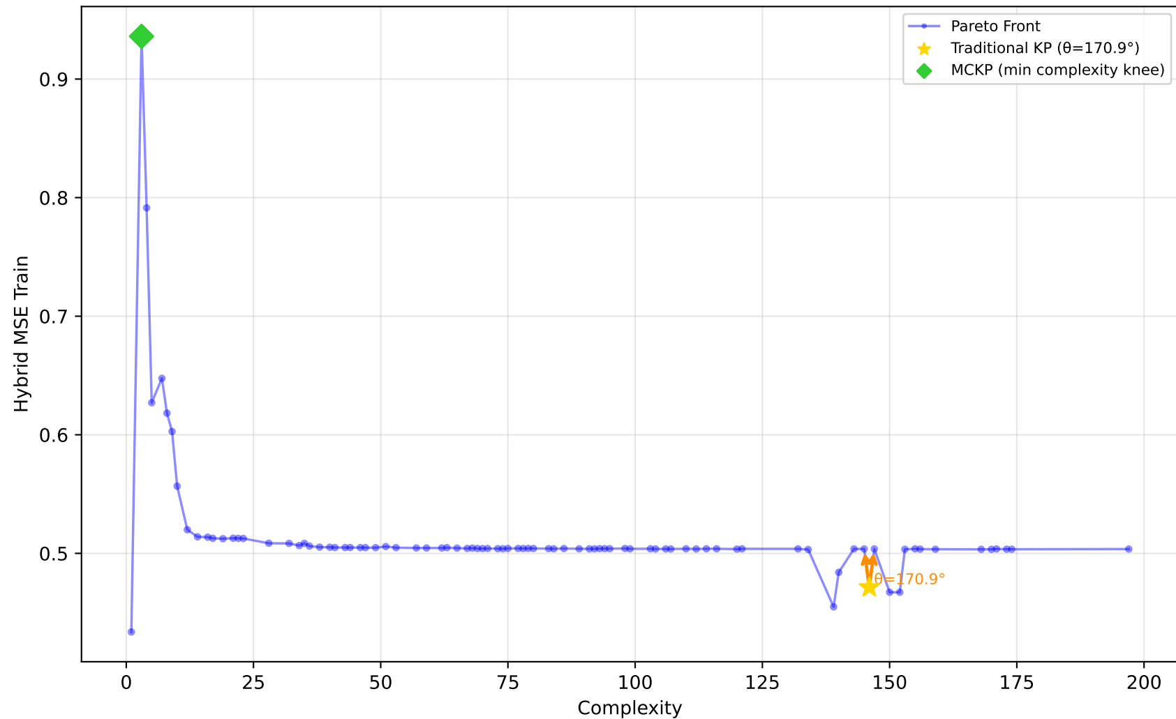
561_cpu - Run 21 - SVP - Hybrid MSE Train \lambda_1=1.00, \lambda_2=0.00, \lambda_3=0.40 | Difficulty: 1.00 | Method: hmr
