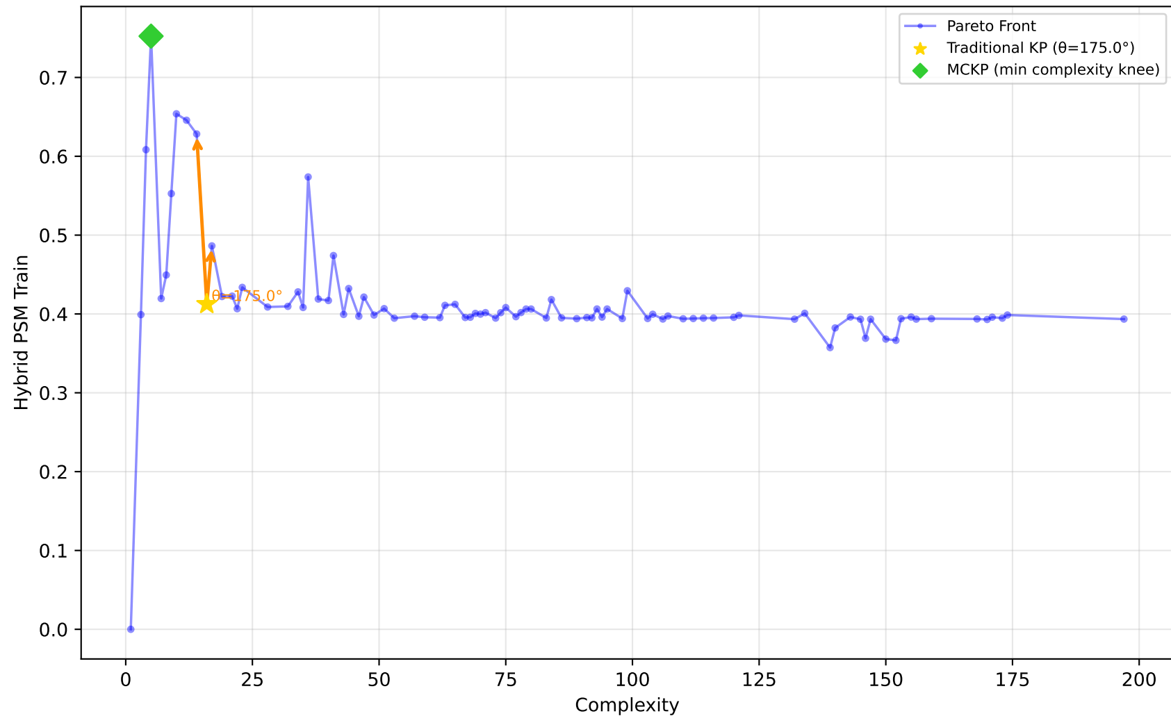
561_cpu - Run 21 - SVP - Hybrid PSM Train \lambda_1=0.90, \lambda_2=0.00, \lambda_3=0.30 | Difficulty: 1.00 | Method: hmr
