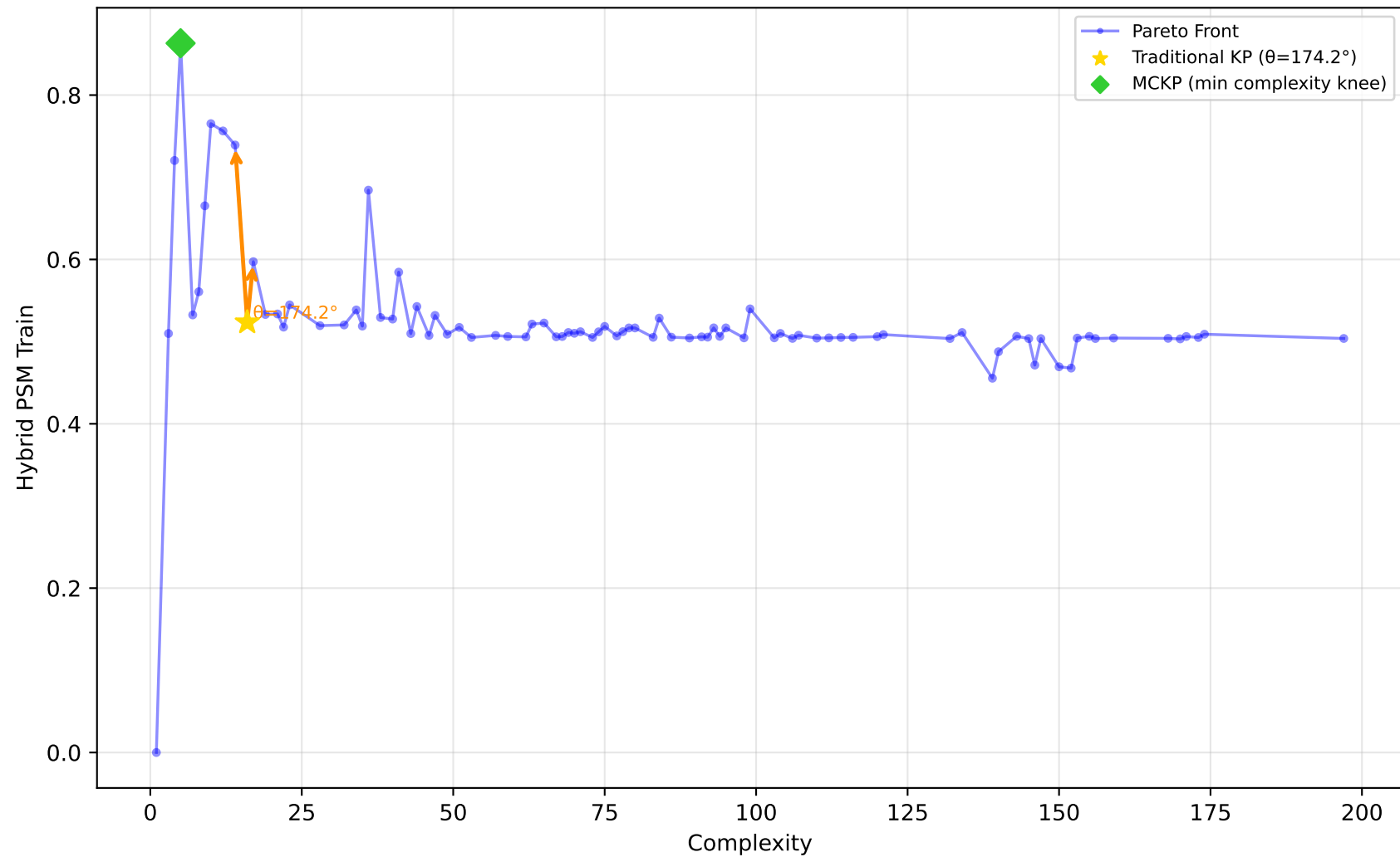
561_cpu - Run 21 - SVP - Hybrid PSM Train \lambda_1=1.00, \lambda_2=0.00, \lambda_3=0.40 | Difficulty: 1.00 | Method: hmr
