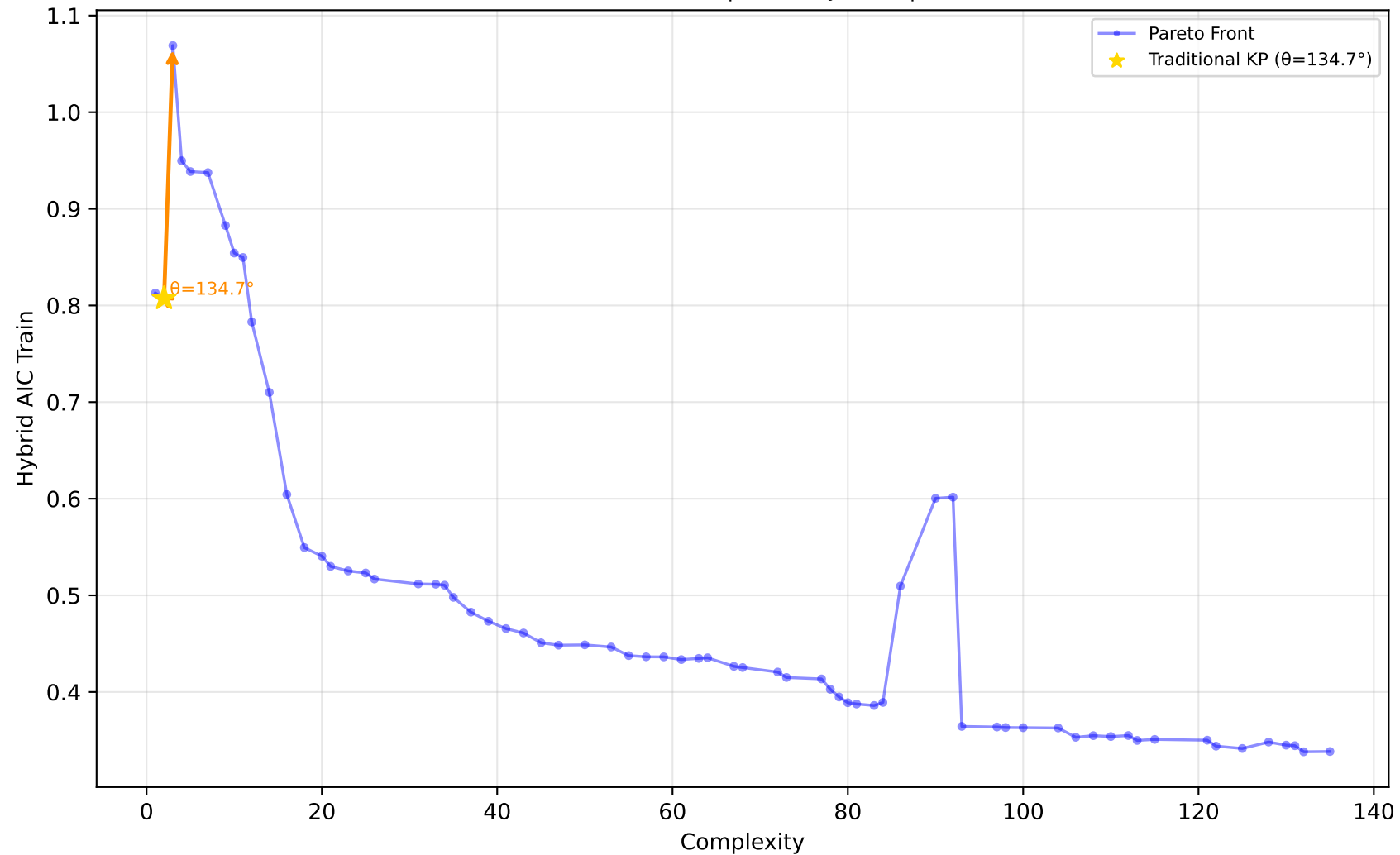
561_cpu - Run 22 - MVP - Hybrid AIC Train \lambda_1=0.50, \lambda_2=0.20, \lambda_3=0.00 | Difficulty: 0.76 | Method: hmr
