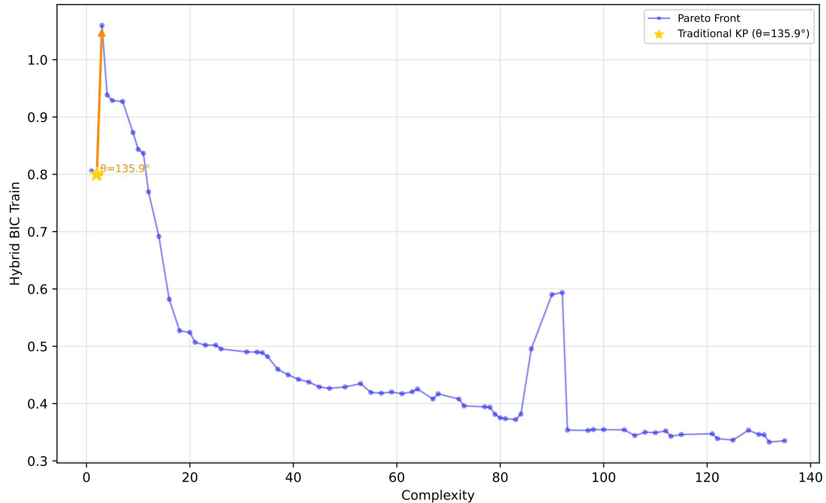
561_cpu - Run 22 - MVP - Hybrid BIC Train \lambda_1=0.50, \lambda_2=0.20, \lambda_3=0.00 | Difficulty: 0.76 | Method: hmr
