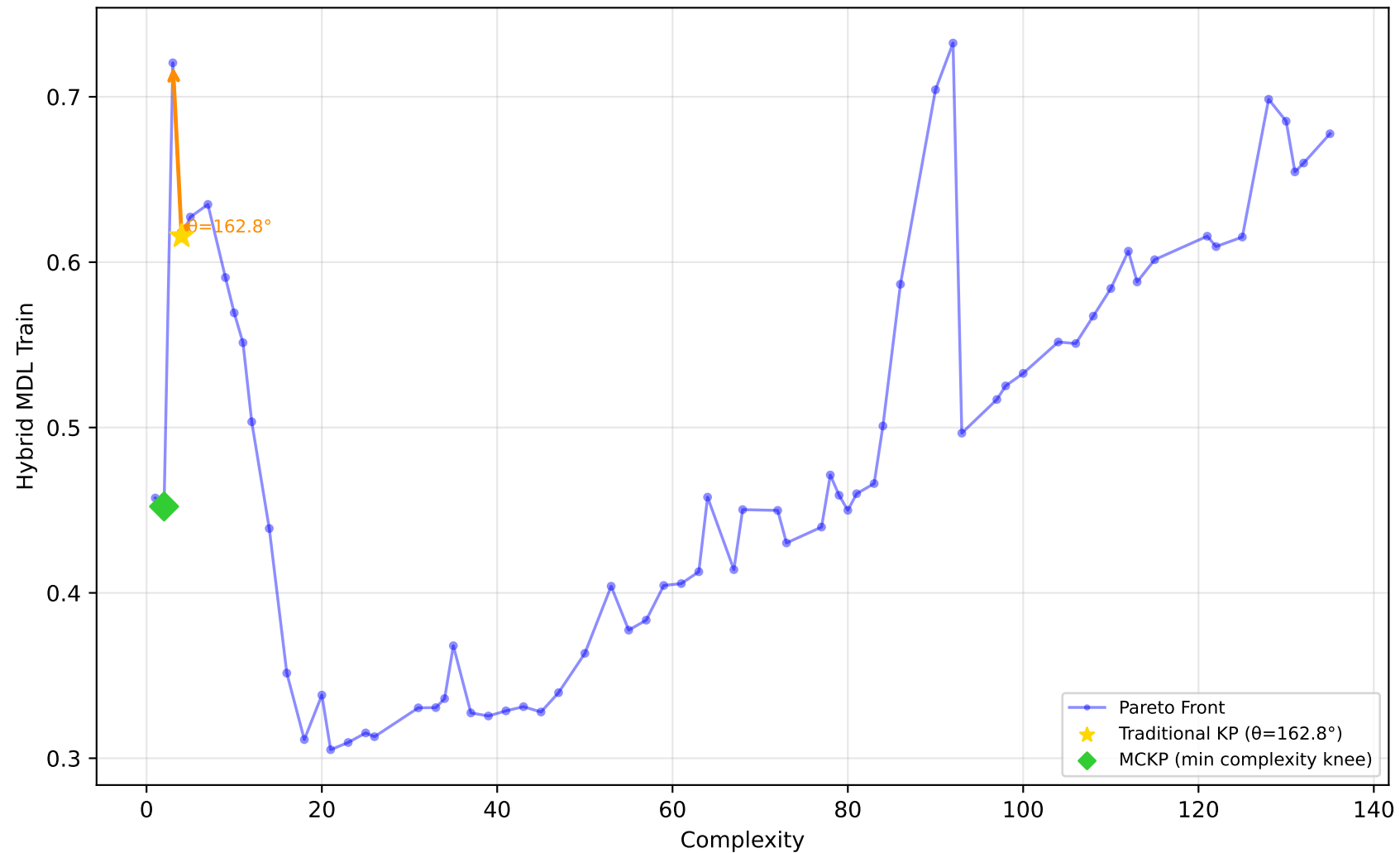
561_cpu - Run 22 - MVP - Hybrid MDL Train \lambda_1=0.50, \lambda_2=0.20, \lambda_3=0.00 | Difficulty: 0.76 | Method: hmr
