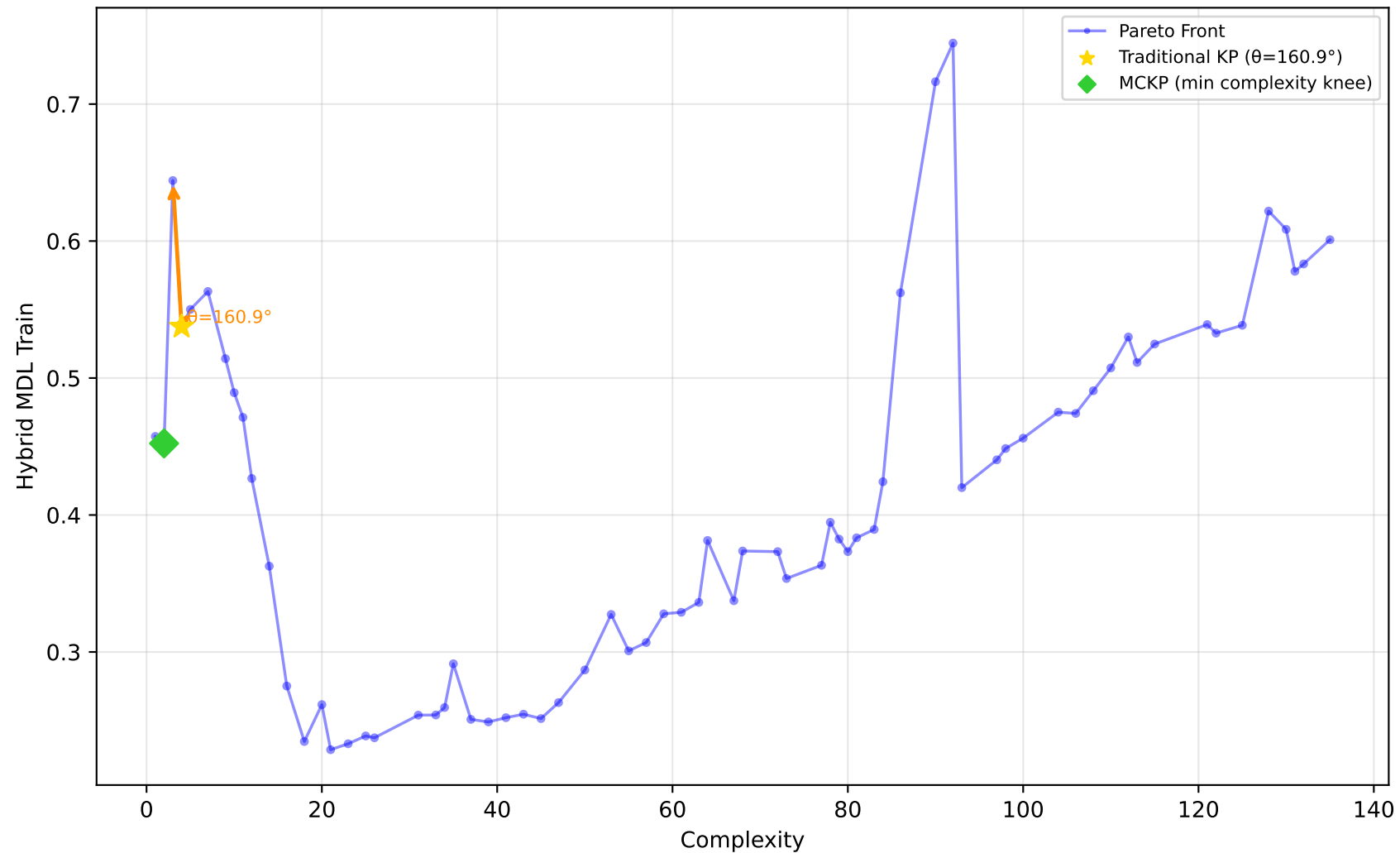
561_cpu - Run 22 - MVP - Hybrid MDL Train \lambda_1=0.70, \lambda_2=0.00, \lambda_3=0.10 | Difficulty: 0.76 | Method: hmr
