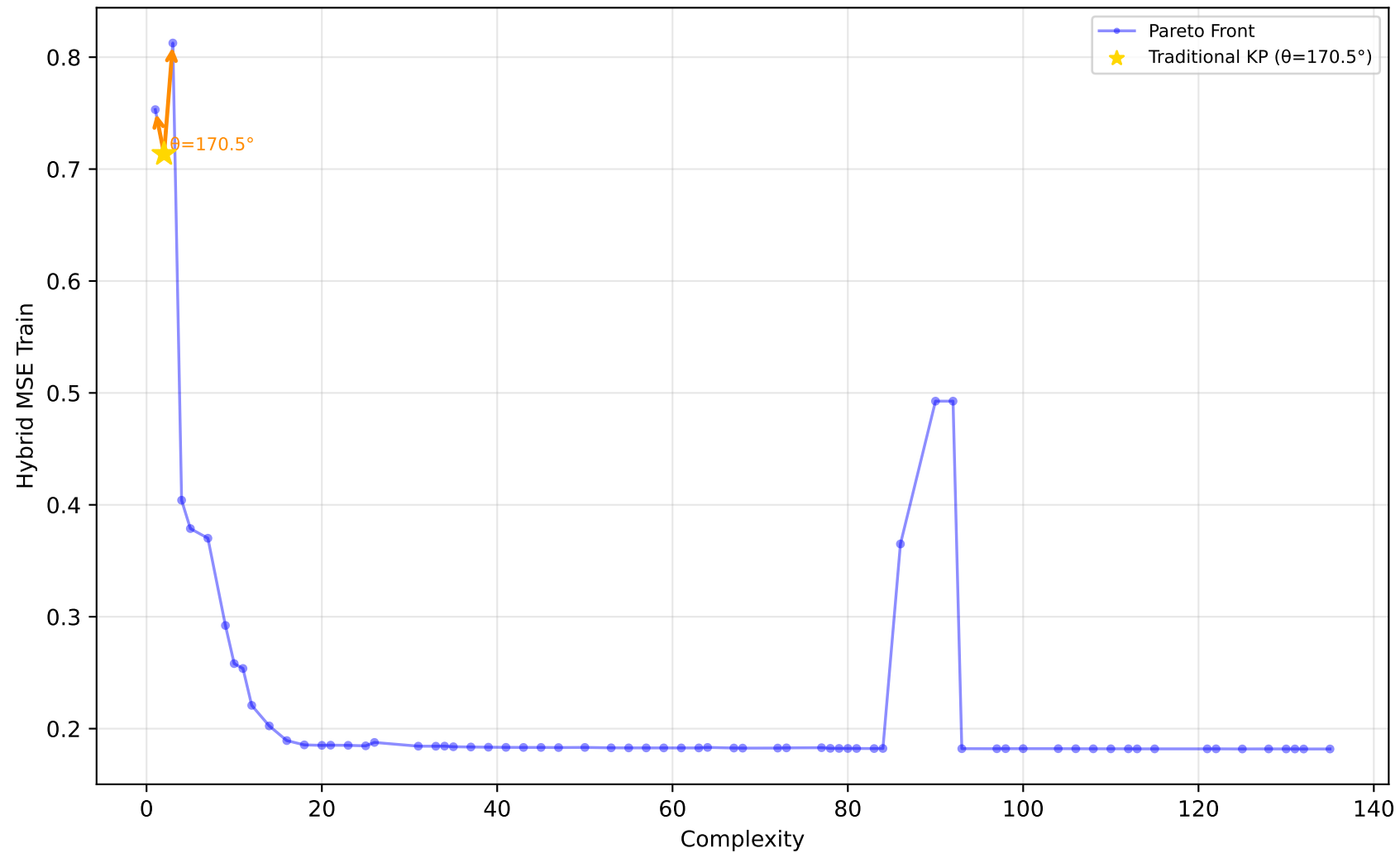
561_cpu - Run 22 - MVP - Hybrid MSE Train \lambda_1=0.70, \lambda_2=0.00, \lambda_3=0.10 | Difficulty: 0.76 | Method: hmr
