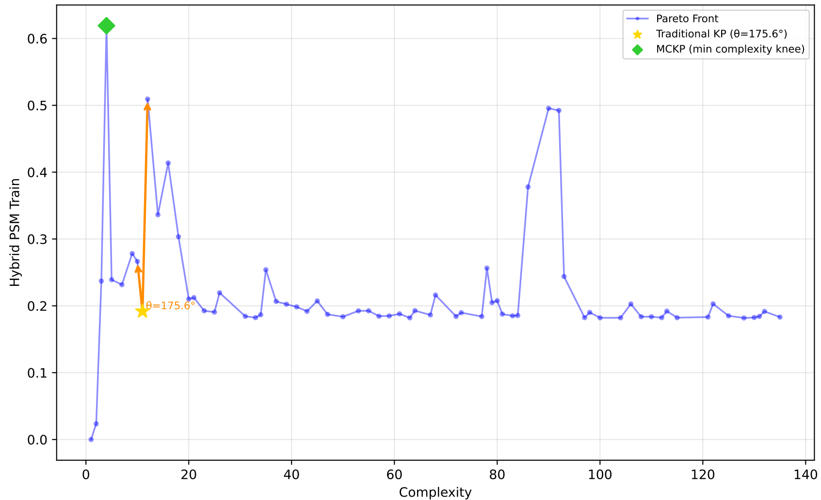
561_cpu - Run 22 - MVP - Hybrid PSM Train \lambda_1=0.70, \lambda_2=0.00, \lambda_3=0.10 | Difficulty: 0.76 | Method: hmr
