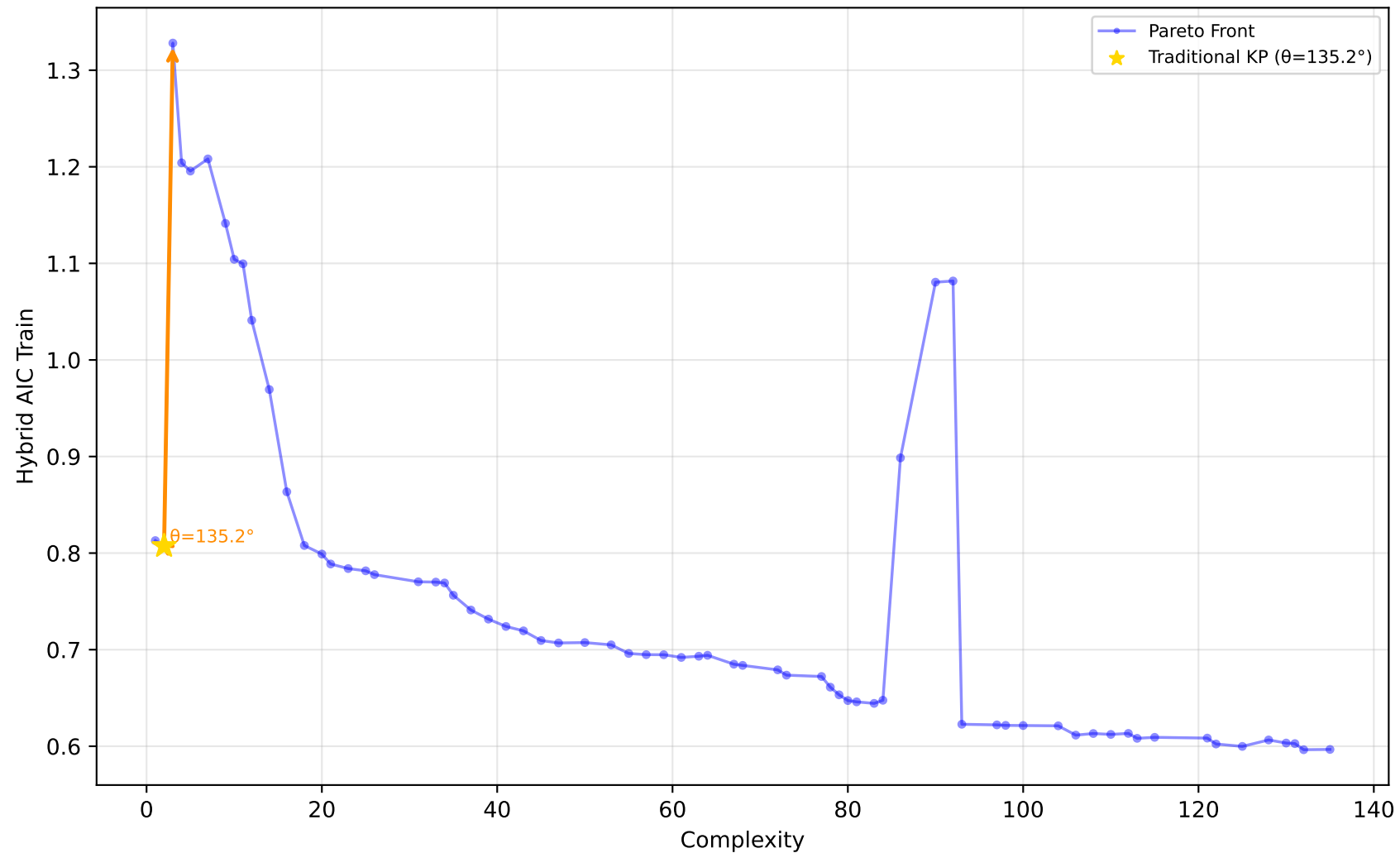
561_cpu - Run 22 - SVP - Hybrid AIC Train \lambda_1=1.00, \lambda_2=0.00, \lambda_3=0.40 | Difficulty: 0.76 | Method: hmr
