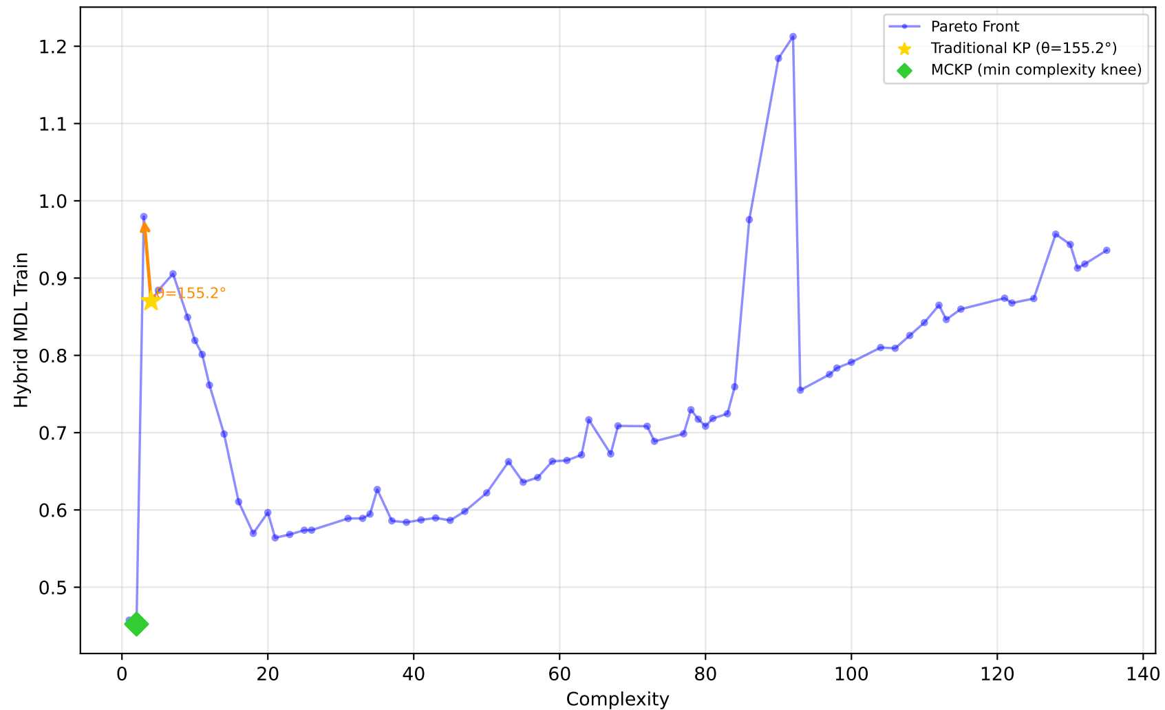
561_cpu - Run 22 - SVP - Hybrid MDL Train \lambda_1=1.00, \lambda_2=0.00, \lambda_3=0.40 | Difficulty: 0.76 | Method: hmr
