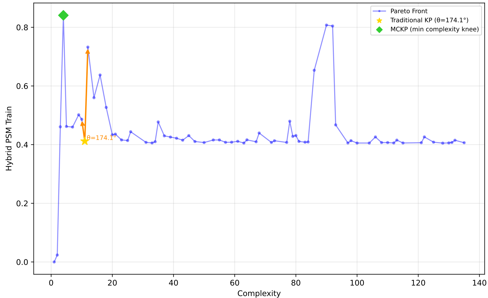
561_cpu - Run 22 - SVP - Hybrid PSM Train \lambda_1=0.90, \lambda_2=0.00, \lambda_3=0.30 | Difficulty: 0.76 | Method: hmr
