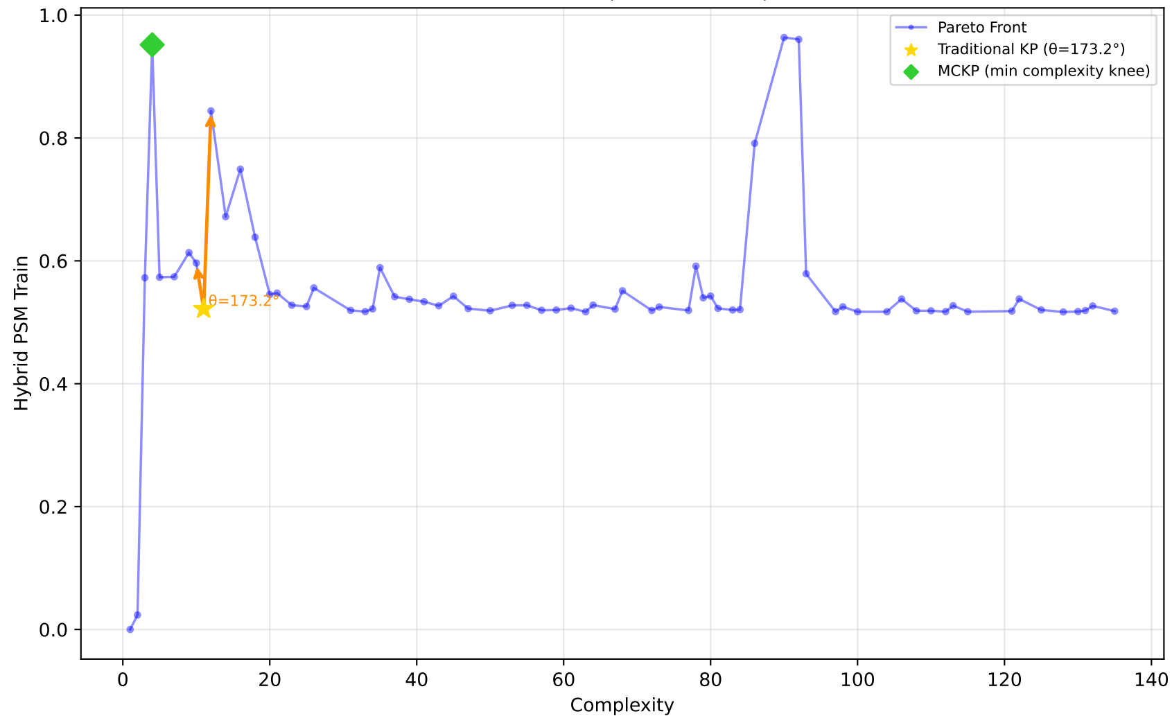
561_cpu - Run 22 - SVP - Hybrid PSM Train \lambda_1=1.00, \lambda_2=0.00, \lambda_3=0.40 | Difficulty: 0.76 | Method: hmr
