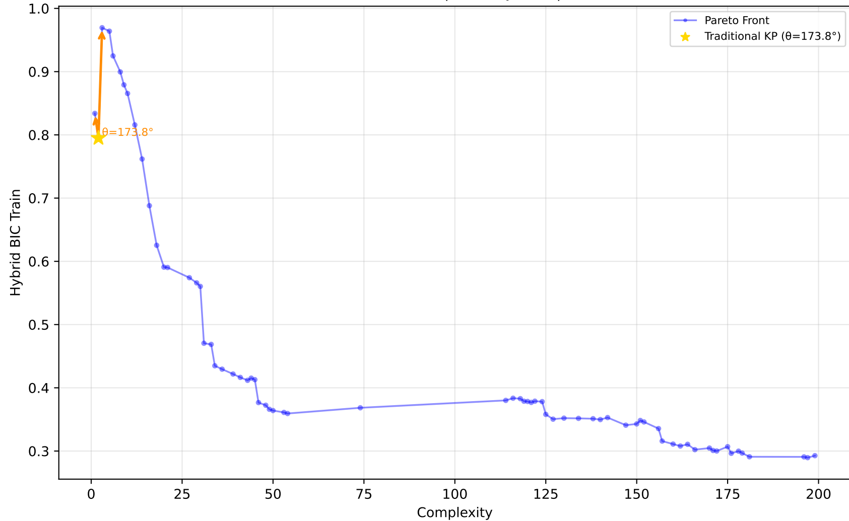
561_cpu - Run 23 - MVP - Hybrid BIC Train \lambda_1=0.50, \lambda_2=0.20, \lambda_3=0.00 | Difficulty: 1.00 | Method: hmr
