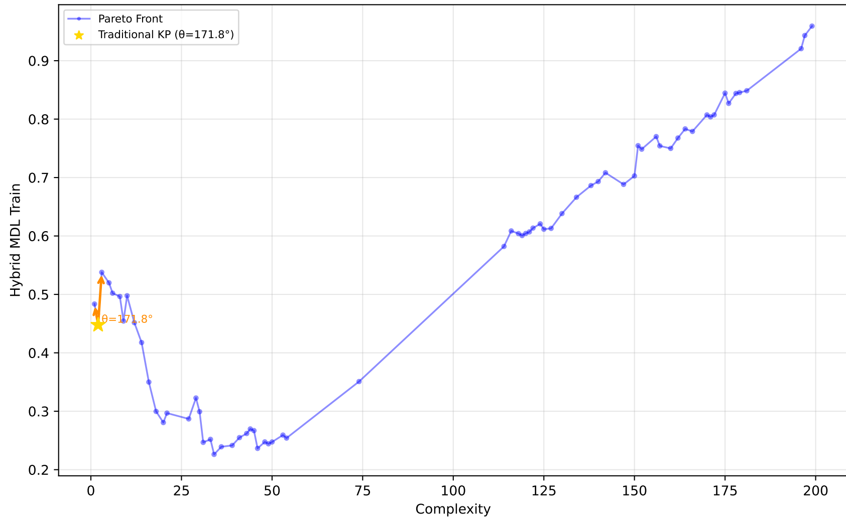
561_cpu - Run 23 - MVP - Hybrid MDL Train \lambda_1=0.70, \lambda_2=0.00, \lambda_3=0.10 | Difficulty: 1.00 | Method: hmr
