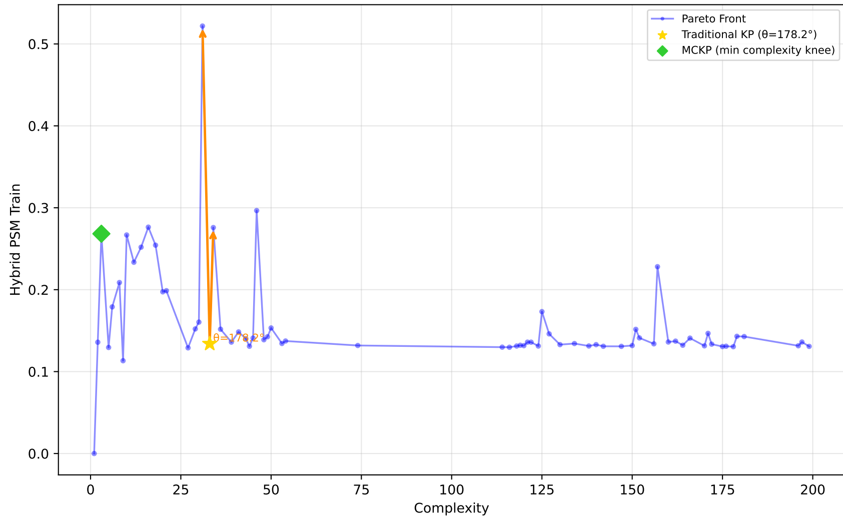
561_cpu - Run 23 - MVP - Hybrid PSM Train \lambda_1=0.70, \lambda_2=0.00, \lambda_3=0.10 | Difficulty: 1.00 | Method: hmr
