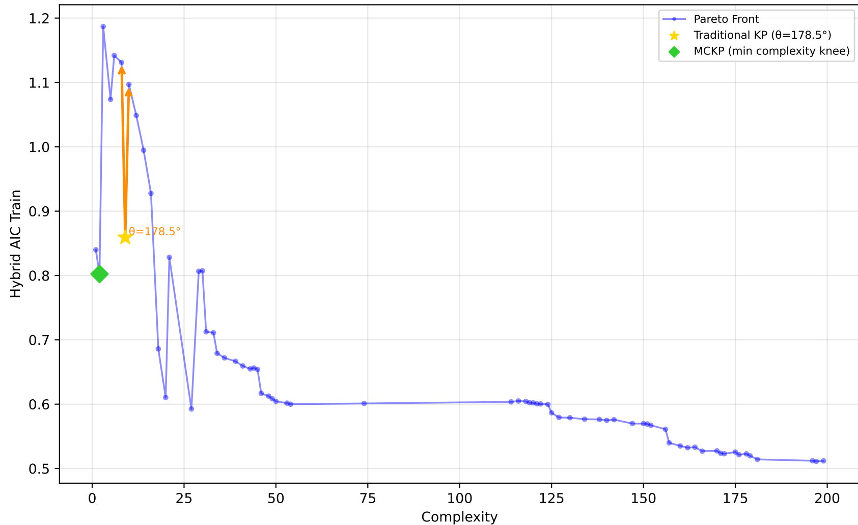
561_cpu - Run 23 - SVP - Hybrid AIC Train \lambda_1=1.00, \lambda_2=0.00, \lambda_3=0.40 | Difficulty: 1.00 | Method: hmr
