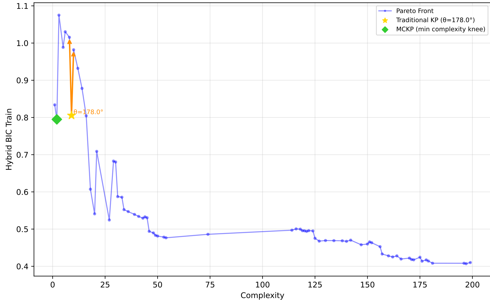
561_cpu - Run 23 - SVP - Hybrid BIC Train \lambda_1=0.90, \lambda_2=0.00, \lambda_3=0.30 | Difficulty: 1.00 | Method: hmr
