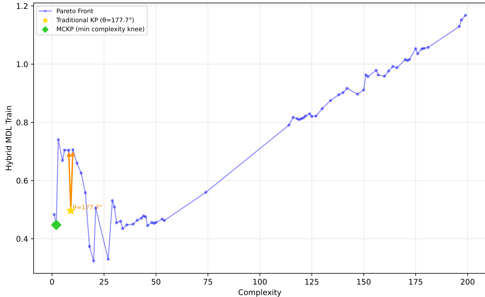
561_cpu - Run 23 - SVP - Hybrid MDL Train \lambda_1=0.90, \lambda_2=0.00, \lambda_3=0.30 | Difficulty: 1.00 | Method: hmr
