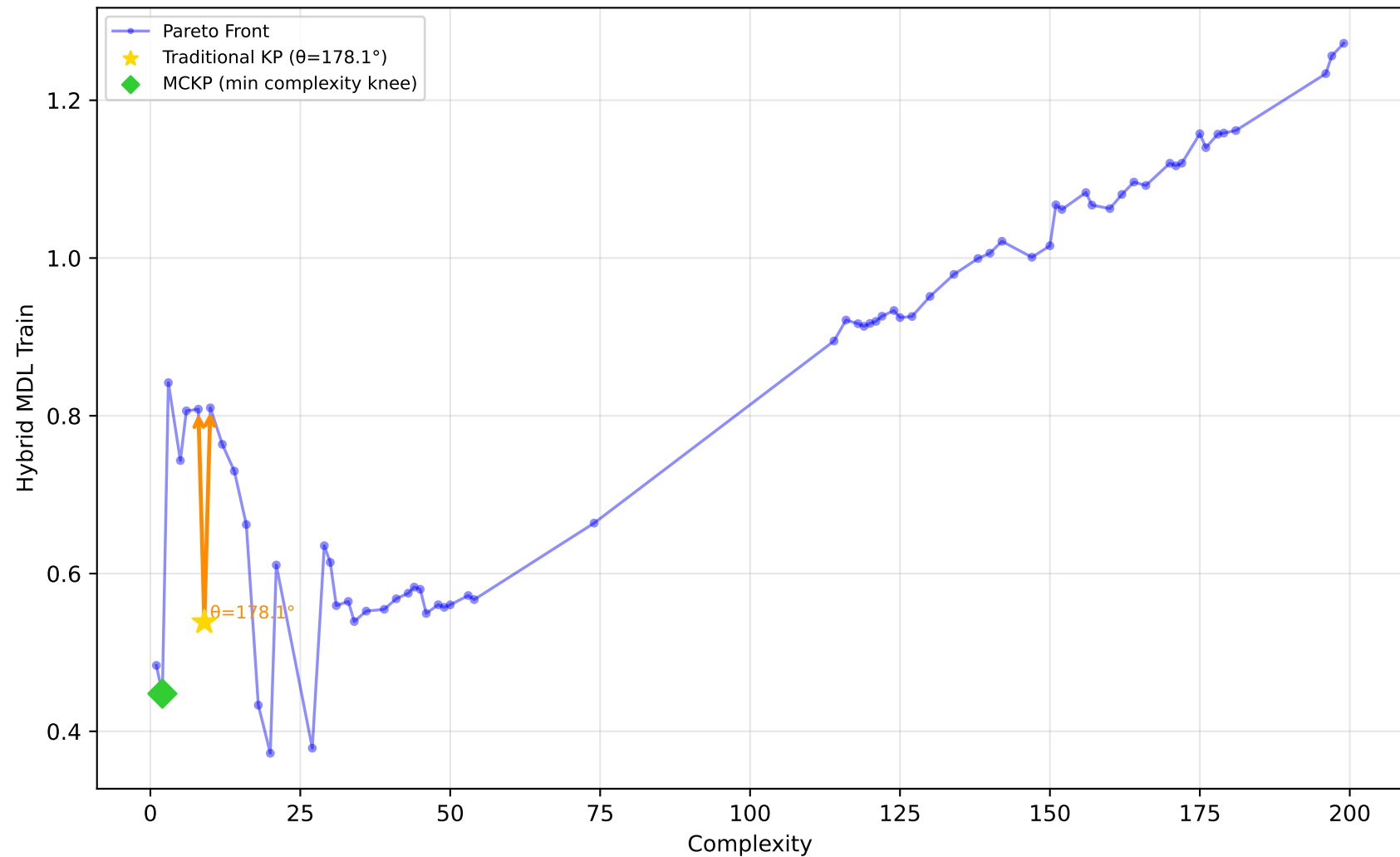
561_cpu - Run 23 - SVP - Hybrid MDL Train \lambda_1=1.00, \lambda_2=0.00, \lambda_3=0.40 | Difficulty: 1.00 | Method: hmr
