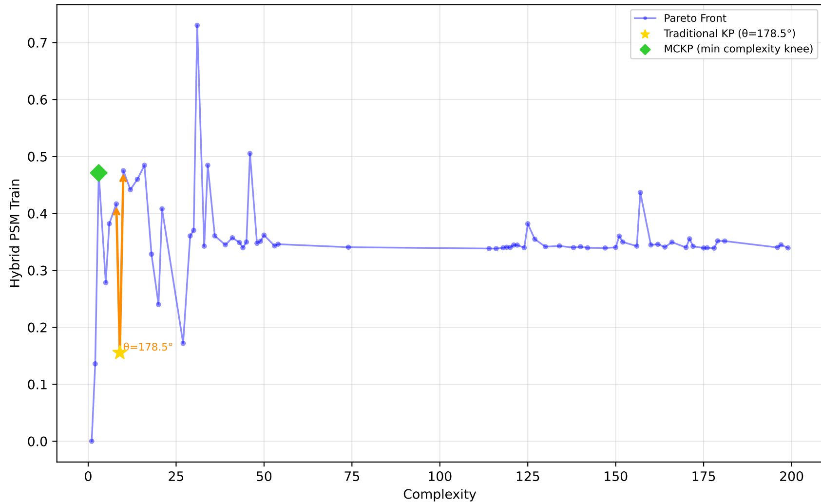
561_cpu - Run 23 - SVP - Hybrid PSM Train \lambda_1=0.90, \lambda_2=0.00, \lambda_3=0.30 | Difficulty: 1.00 | Method: hmr
