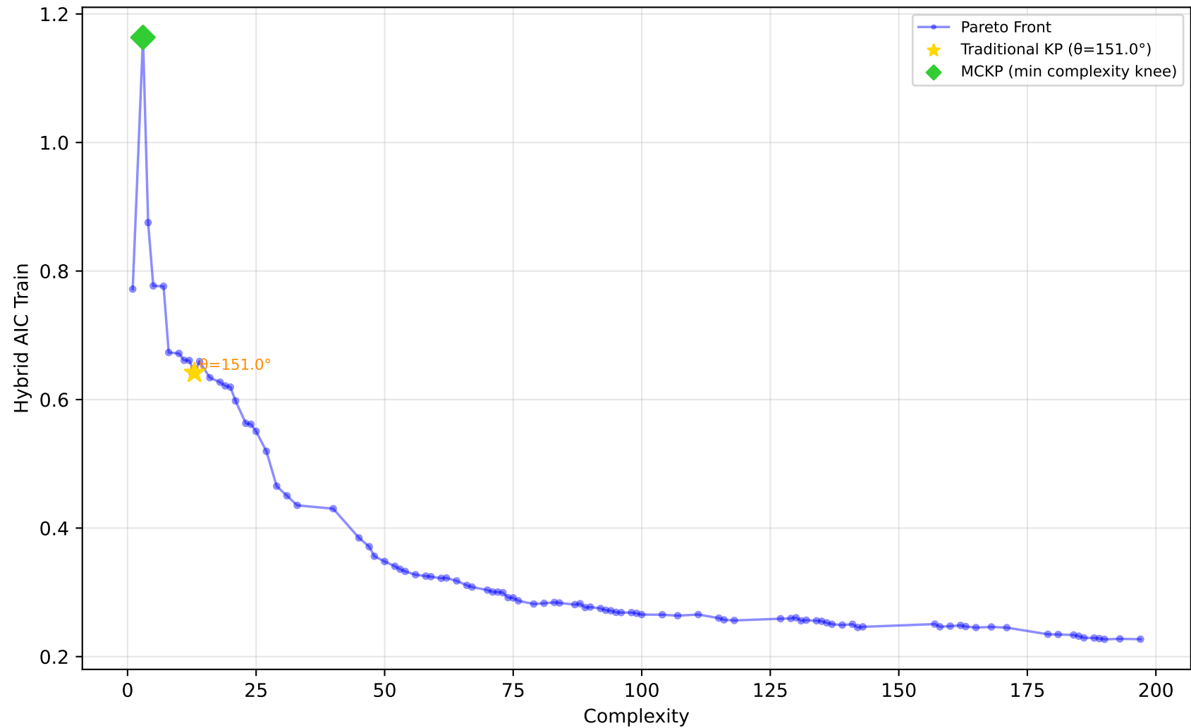
561_cpu - Run 24 - MVP - Hybrid AIC Train \lambda_1=0.70, \lambda_2=0.00, \lambda_3=0.10 | Difficulty: 1.00 | Method: hmr
