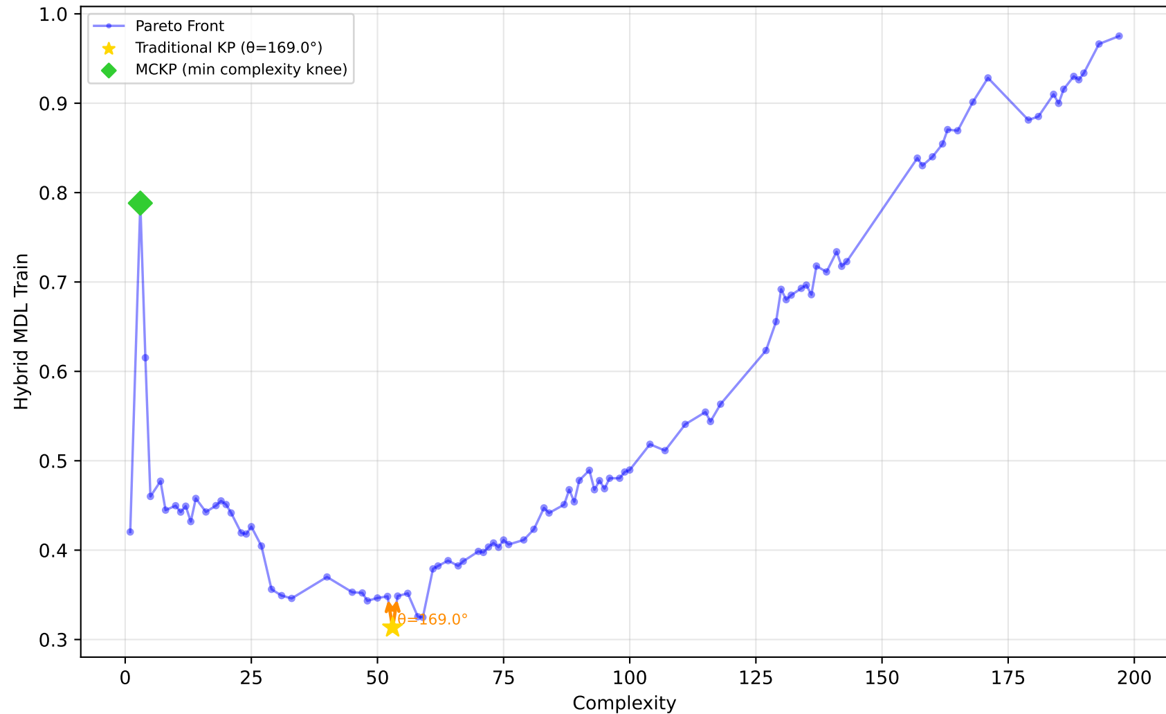
561_cpu - Run 24 - MVP - Hybrid MDL Train \lambda_1=0.50, \lambda_2=0.20, \lambda_3=0.00 | Difficulty: 1.00 | Method: hmr
