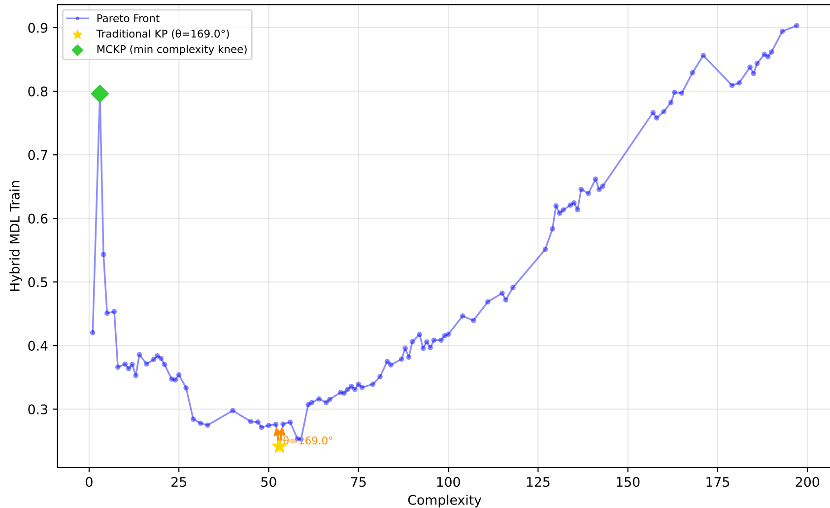
561_cpu - Run 24 - MVP - Hybrid MDL Train \lambda_1=0.70, \lambda_2=0.00, \lambda_3=0.10 | Difficulty: 1.00 | Method: hmr
