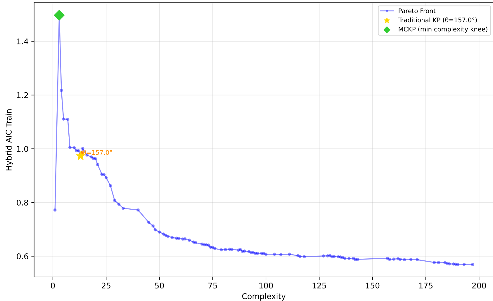
561_cpu - Run 24 - SVP - Hybrid AIC Train \lambda_1=1.00, \lambda_2=0.00, \lambda_3=0.40 | Difficulty: 1.00 | Method: hmr
