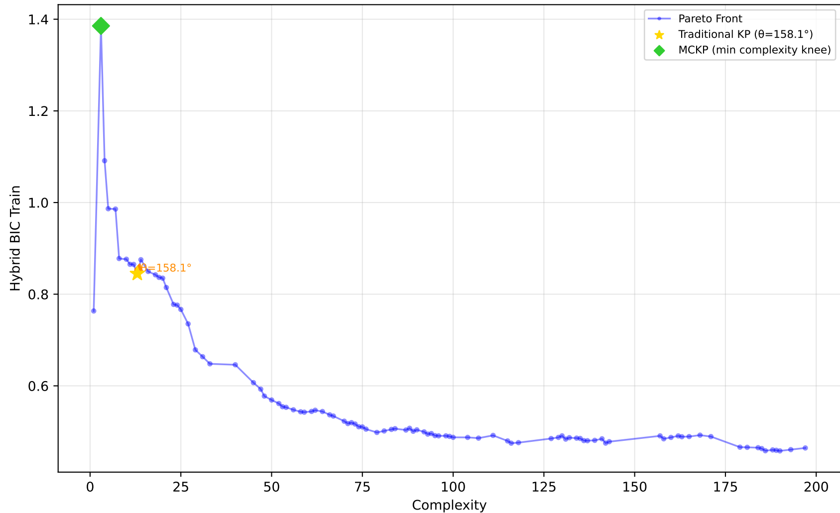
561_cpu - Run 24 - SVP - Hybrid BIC Train \lambda_1=0.90, \lambda_2=0.00, \lambda_3=0.30 | Difficulty: 1.00 | Method: hmr
