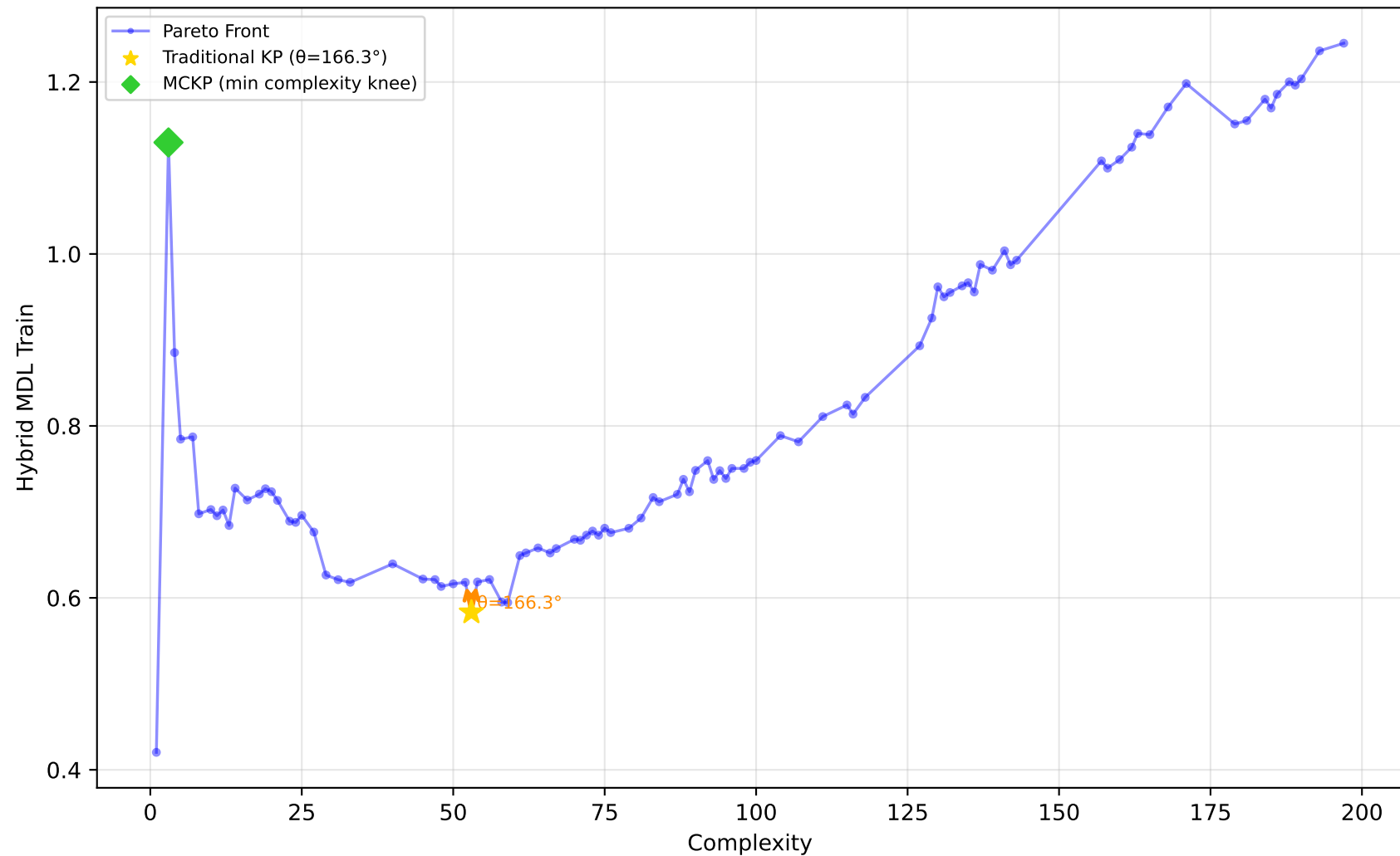
561_cpu - Run 24 - SVP - Hybrid MDL Train \lambda_1=1.00, \lambda_2=0.00, \lambda_3=0.40 | Difficulty: 1.00 | Method: hmr
