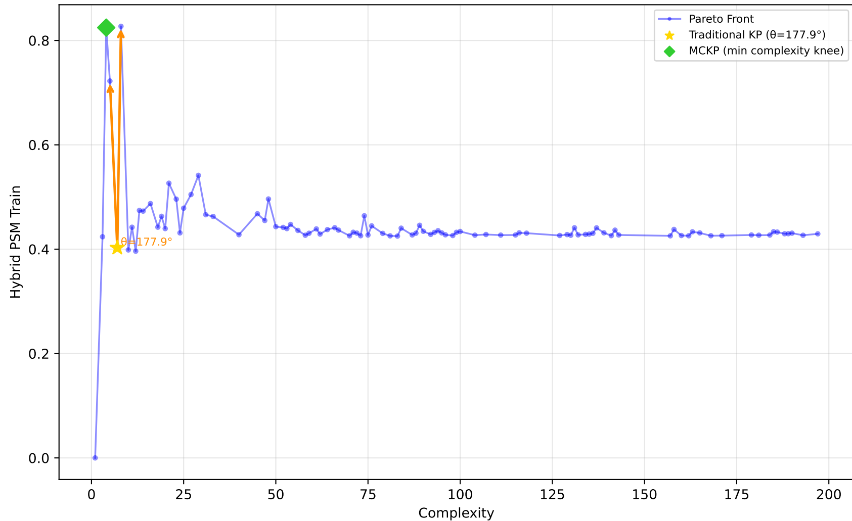
561_cpu - Run 24 - SVP - Hybrid PSM Train \lambda_1=0.90, \lambda_2=0.00, \lambda_3=0.30 | Difficulty: 1.00 | Method: hmr
