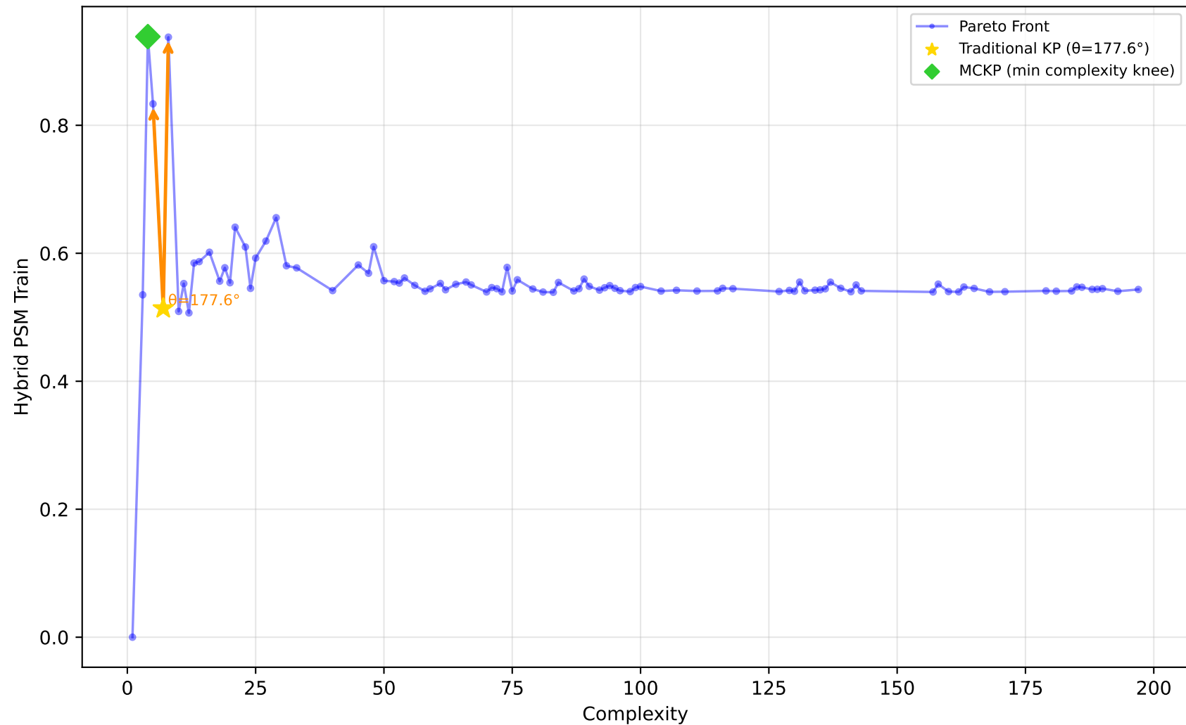
561_cpu - Run 24 - SVP - Hybrid PSM Train \lambda_1=1.00, \lambda_2=0.00, \lambda_3=0.40 | Difficulty: 1.00 | Method: hmr
